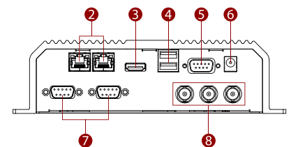
2 LAN 3 HDMI 4 USB Type-A 5 COM 6 Power Input 7 COM (Optional) 8 CVBS Input (Optional)
