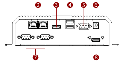
2 LAN 3 HDMI 4 USB Type-A 5 COM 6 Power Input 7 COM (Optional) 8 HDMI Input (Optional)
