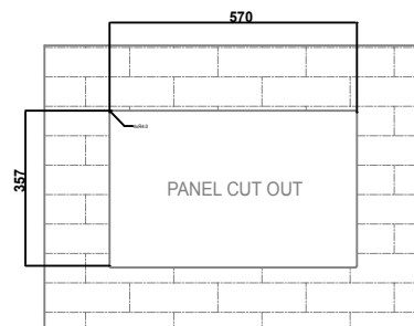
CUT OUT DIMENSION
