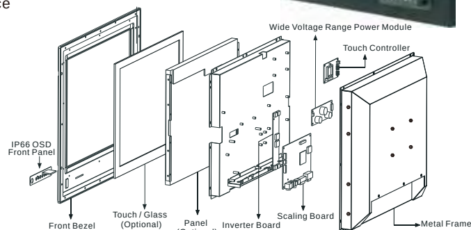
Modularized Construction
