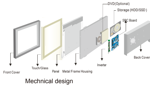
Mechanical design
