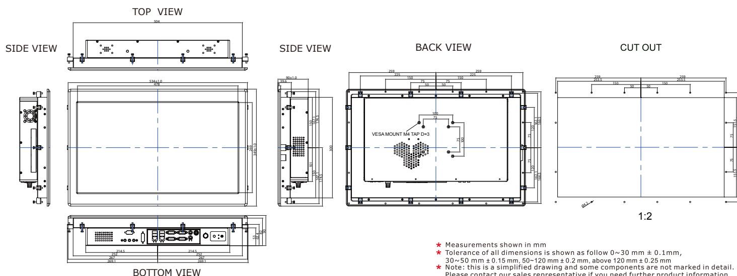
Mechanical Design Dimensions
