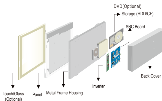
Mechanical design
