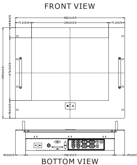
Rack Mount
