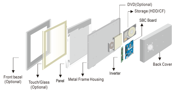
Modularized Construction
