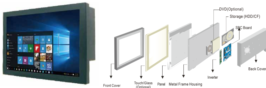
Mechanical design
