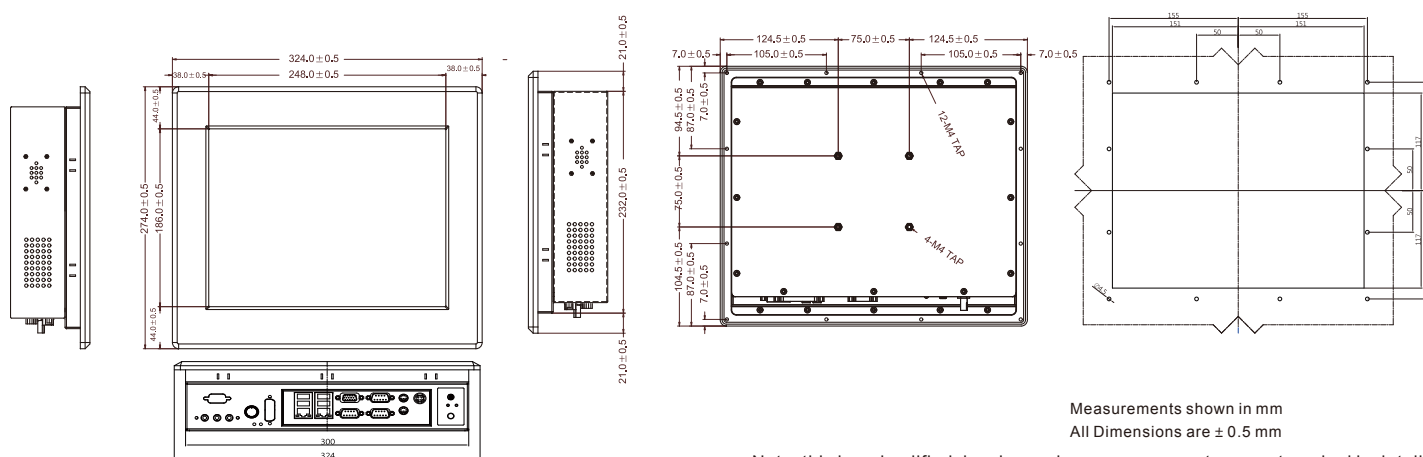
IP65 CUT OUT
