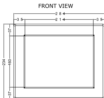
Panel Mount (6 mm front bezel)
