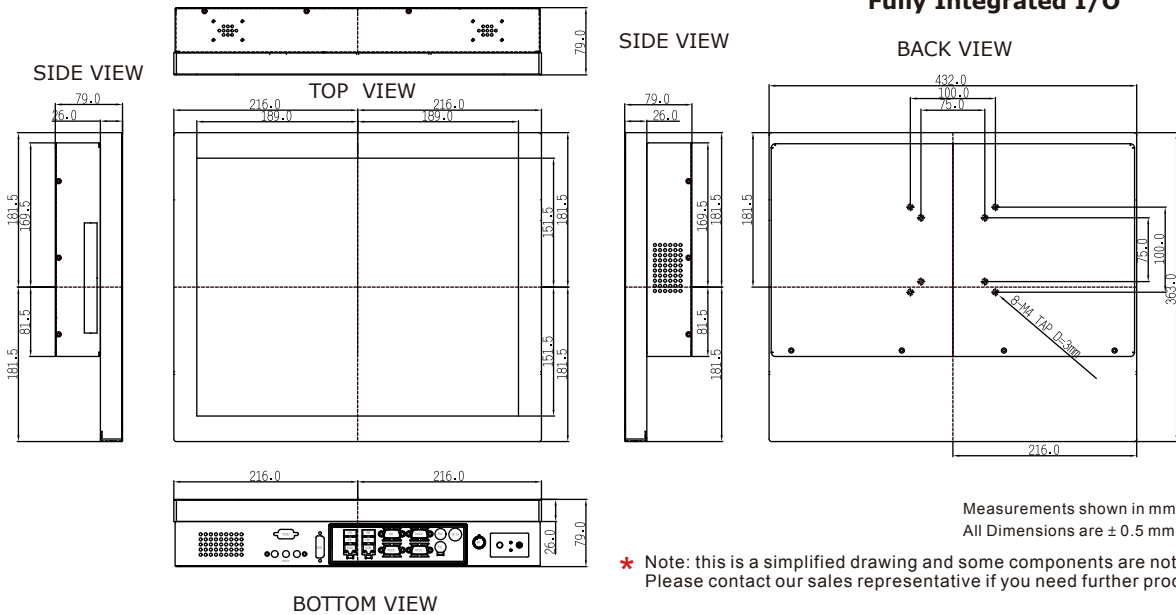
BOTTOM VIEW
