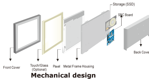
Mechanical design
