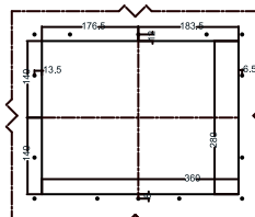
IP65 CUT OUT
