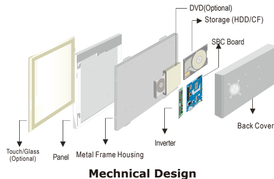
Mechanical Design
