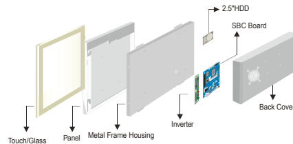
Modularized Construction
