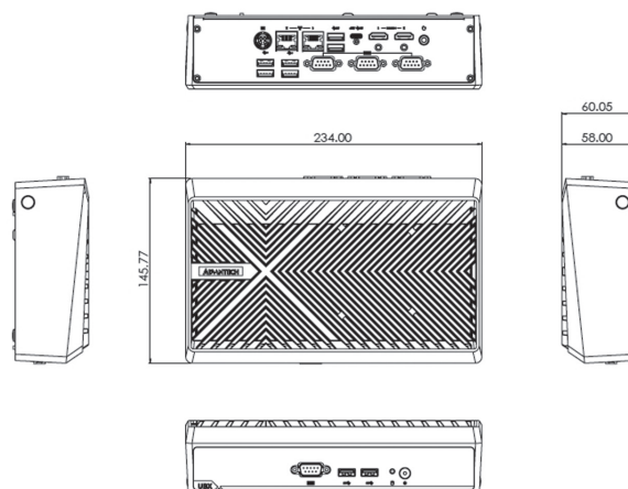
UBX-210H with I/O Type B
