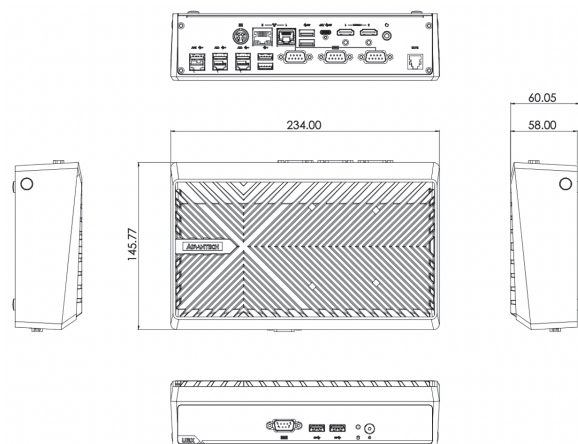
UBX-210H with I/O Type A
