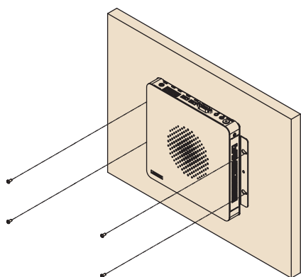
Wall Mount
