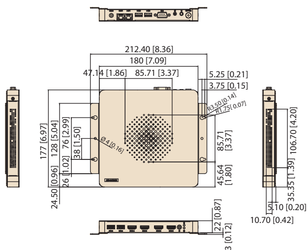
Wall Mount
