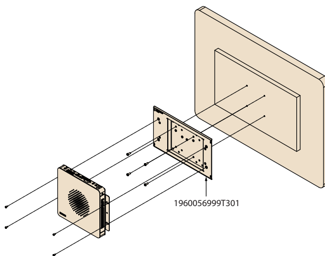
VESA Mount
