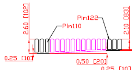
Detail D
