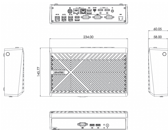
UBX-210K with I/O Type A
