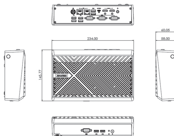
UBX-210K with I/O Type B
