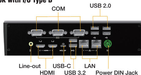
UBX-210K with I/O Type B
