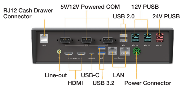
UBX-210K with I/O Type B
