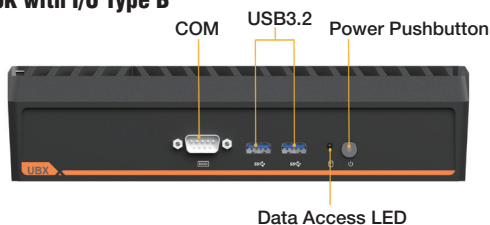
UBX-210K with I/O Type B
