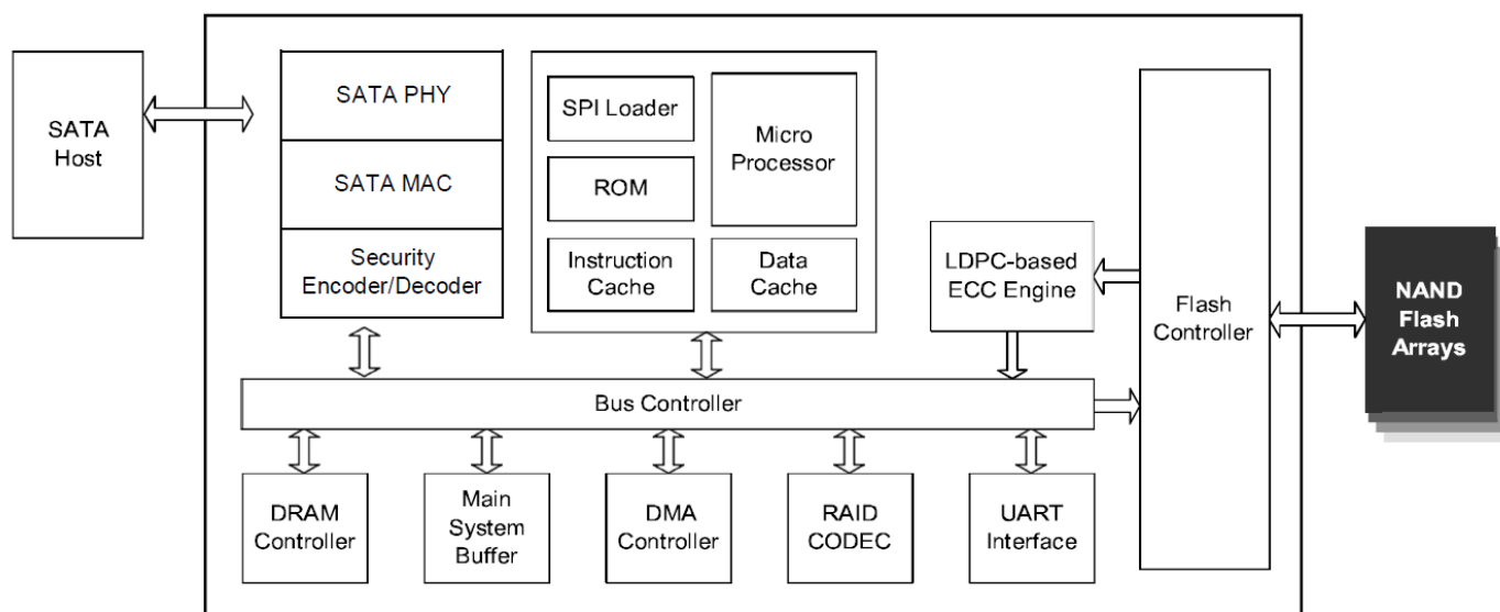
Figure 1-1 Functional Block
