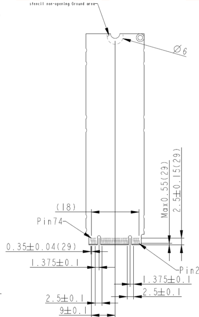
Top View, Bottom side
