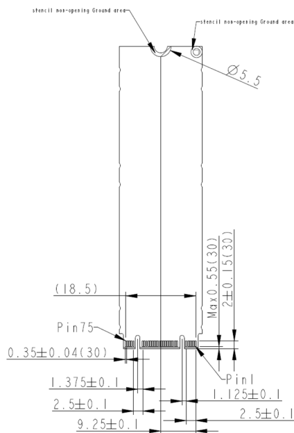
Top View, Top side
