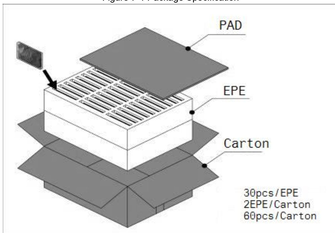
Figure 7-1 Package Specification
