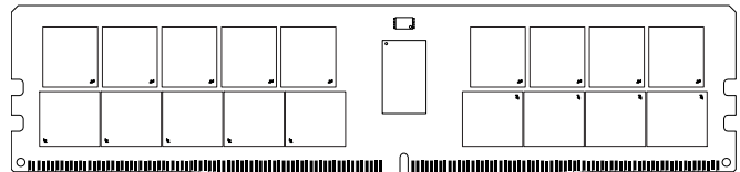
Figure 1: 288-Pin RDIMM (MO-309, R/C-B3)
