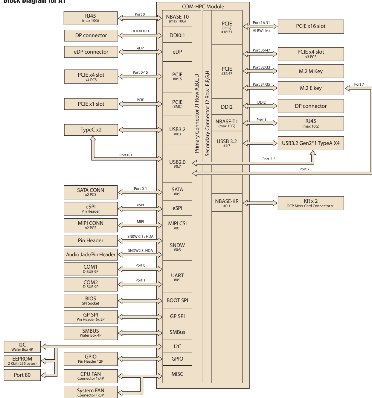
Block Diagram for A1
