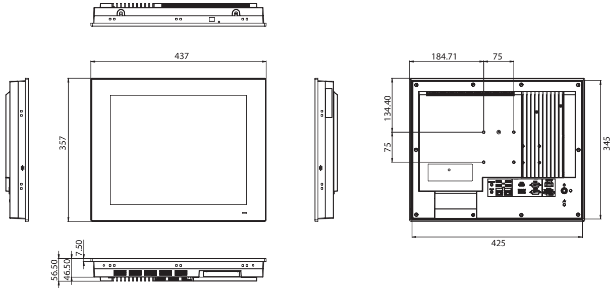
Panel Cutout Dimensions: 427 x 347 mm (16.81 x 13.66 in)
