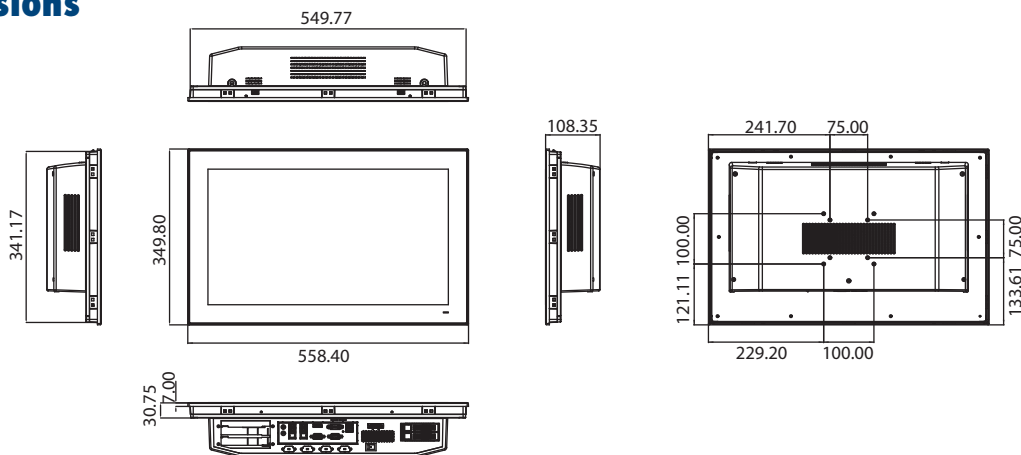
Panel Cutout Dimensions: 550.3 x 341.8 mm (21.66 x 13.45 in)
