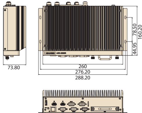
ARK-2250R
