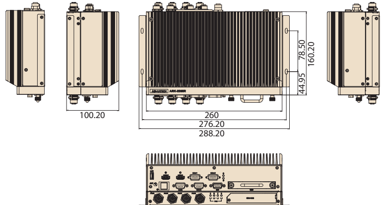
ARK-2250R+AMK-R100E
