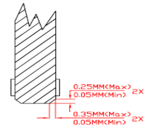
VIEW C-C
