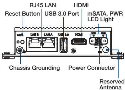
UNO-2271G-E21AE
