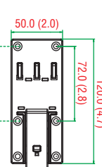
DIN-Rail Mounting Kit
